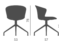
Telaio 4 gambe 4 legs frame AN Vern. nero / Black painted AV Vern. alluminio / Aluminium painted AB Vern. bianco / White painted ACC Cromato / Chromed frame
