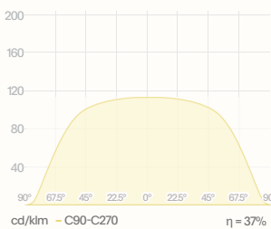
Light distribution for dark fabric Golf LED
