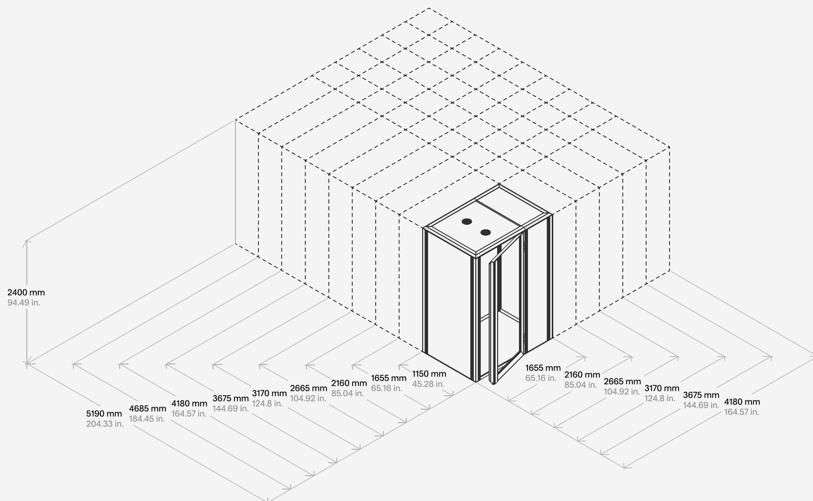
Dimensions duplication scheme (mm) for closed rooms
