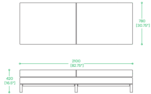
ARC/32 Large Bench
