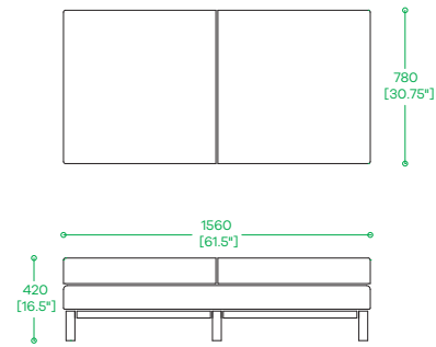
ARC/31 Compact Bench
