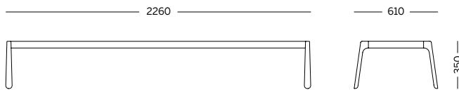
MODULE D - Structure for 4 units
