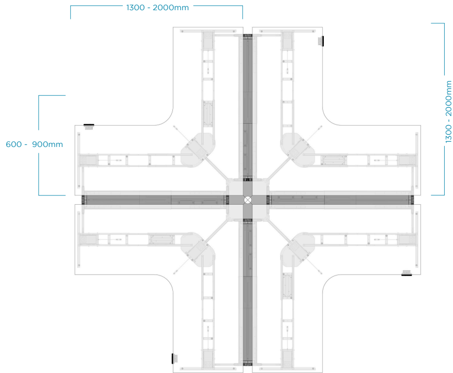
90° Cluster Dimensions
