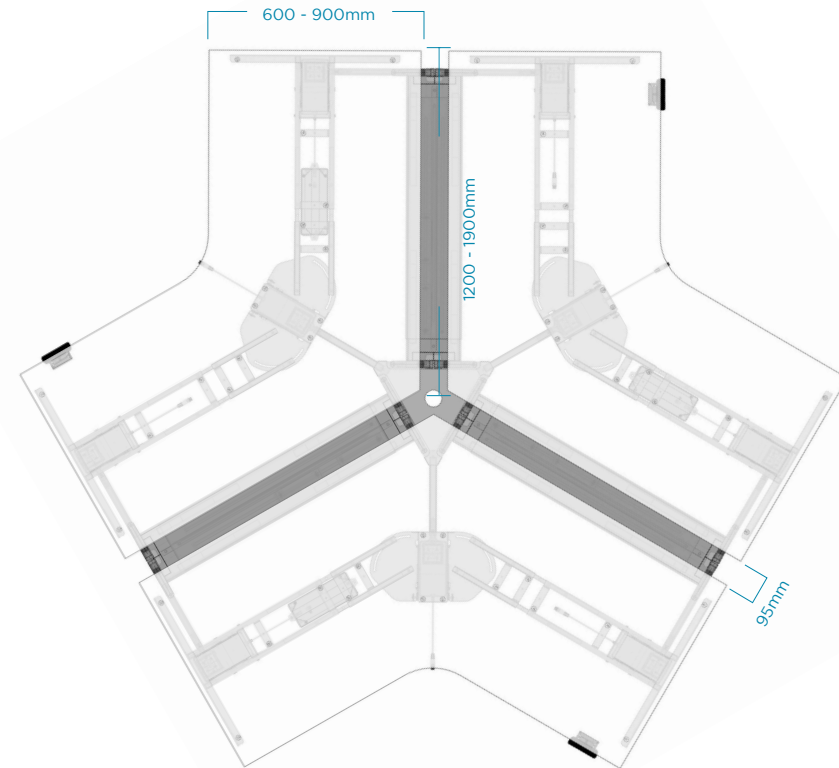
120° Cluster Dimensions
