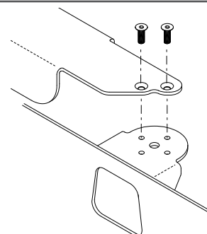
RAIL CONNECTIONS (STANDARD ON ALL DRUM BASES)
