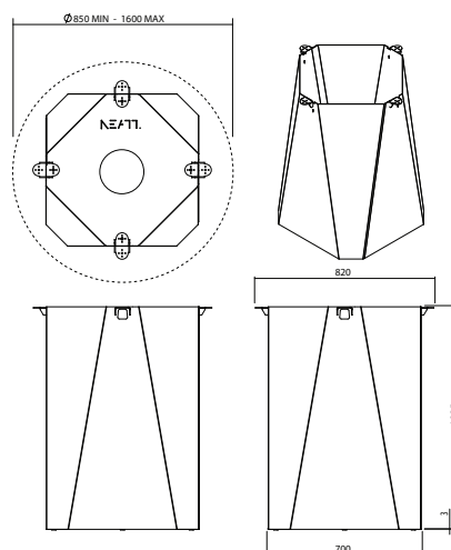
NT-PET-700-1025 Weight: 66kg
