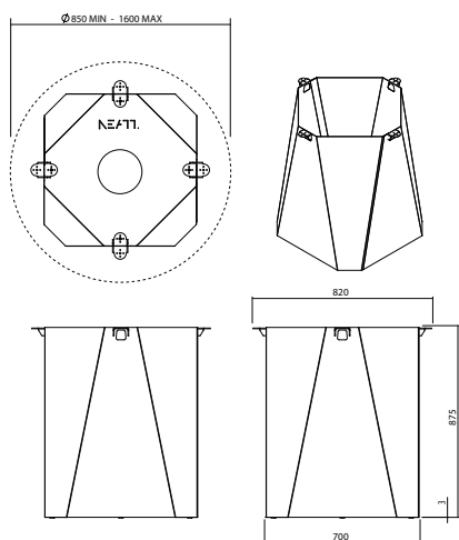
NT-PET-700-875 Weight: 61kg
