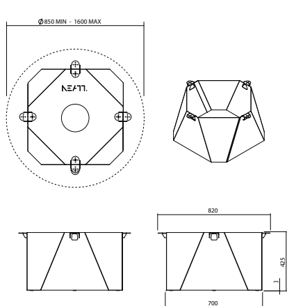
NT-PET-700-425 Weight: 33kg
