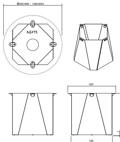
NT-PET-700-715 Weight: 49kg
