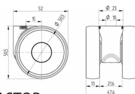
NT-ARC-CASTOR 4 SET OF TENETE LINEA CASTORS (COMPATIBLE WITH WEIGHT PLATES)
