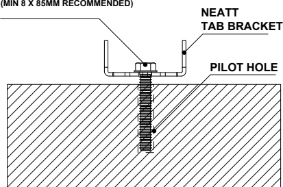
FLOOR FIX (TYPICAL DETAIL)
