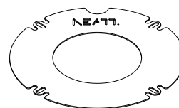
NT-DOL- WPT-700 WEIGHT PLATE - 12kg (TO SUIT 700MM DIAMETER BASE)
