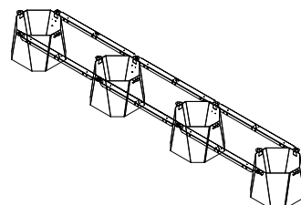
NT-PET-500-425X4 suits - 4800 x 1200mm
