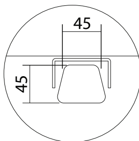
POWER AND DATA CUTOUTS (STANDARD ON ALL DRUM BASES)
