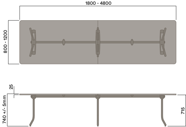
EPT-1040 3 Leg Table 740mm (standard height)
