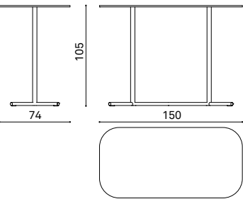
NTT150105 high rectangular table h105 cm tavolo alto rettangolare h105 cm table haute rectangulaire h105 cm
