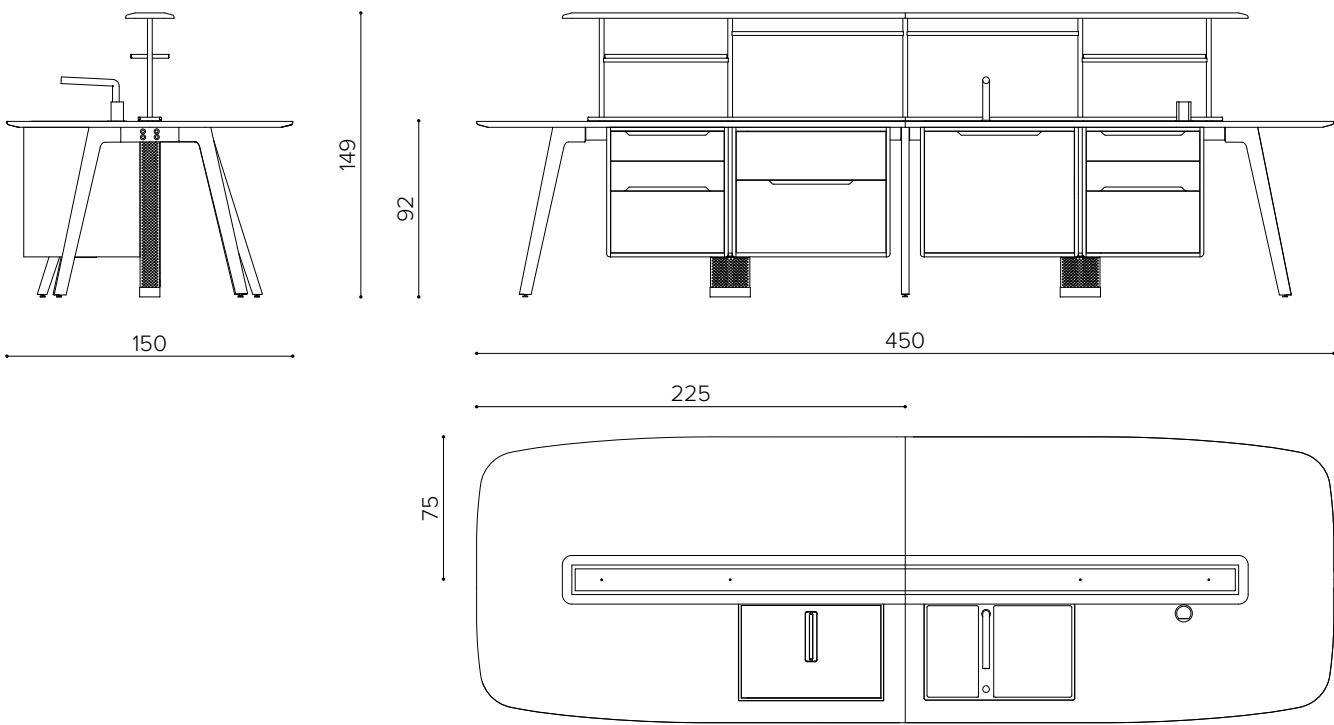
WI 450K Wing kitchen 450x150 standard configuration Wing Kitchen 450x150 configurazione standard Wing Kitchen 450x150 configuration standard
