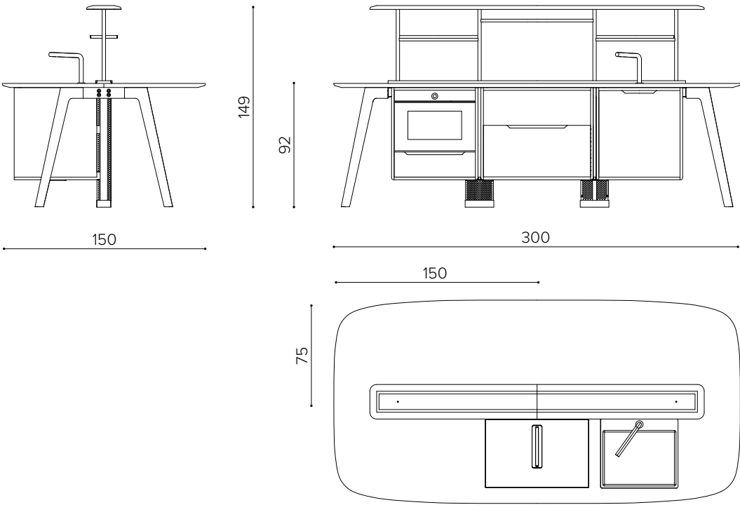
WI 300K Wing kitchen 300x150 standard configuration Wing Kitchen 300x150 configurazione standard Wing Kitchen 300x150 configuration standard
